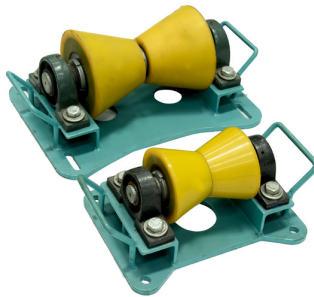
CONE TYPE PIPE ROLLER NYLON
