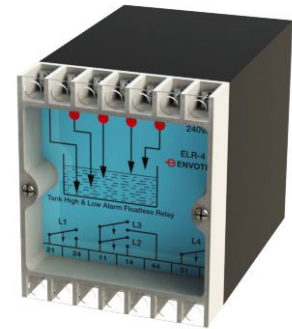
ELR SERIES ELECTRONIC LEVEL RELAY
